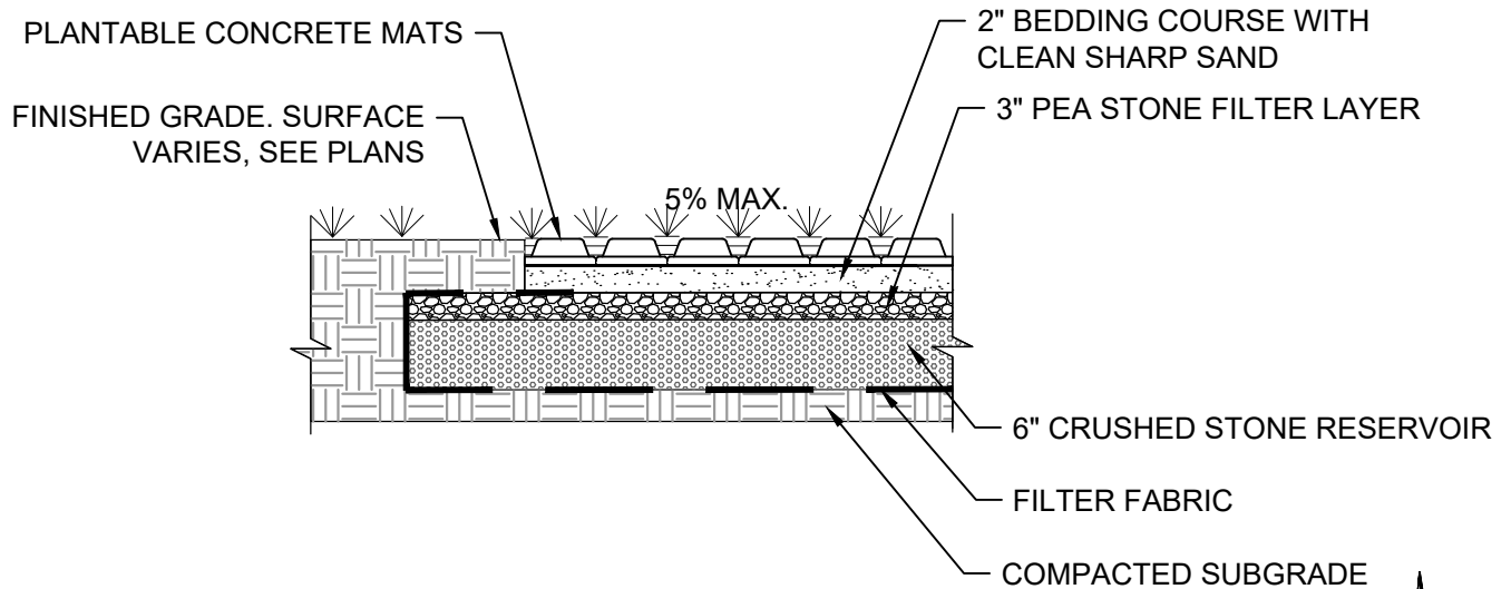
PERMEABLE PAVER DETAIL NOT TO SCALE
