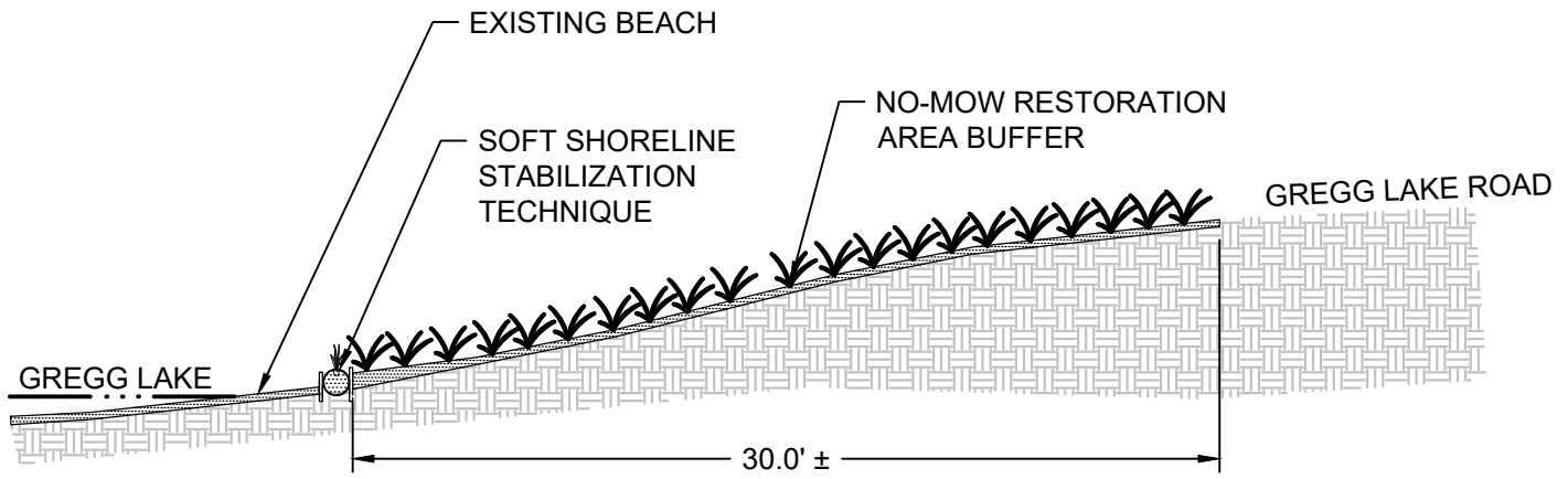
RESTORATION AREA CROSS SECTION NOT TO SCALE
