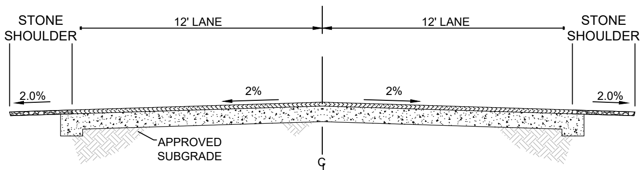
TYPICAL 2-LANE ROADWAY CROSS SECTION CROWNED-OPEN SECTION NOT TO SCALE
