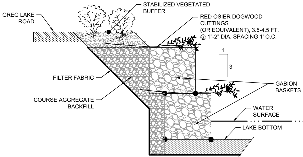
GABION WALL WITH VEGETATED BUFFER NOT TO SCALE
