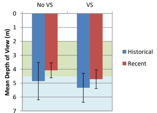
Figure 4.5.2. Mean historical and recent SDT measured with (VS) or without (No VS) a viewscope as shown in Table 4.5.1. The blue shaded area indicates SDT depths considered “Exceptional” and the green shaded area is considered “Good.” Error bars represent standard deviations for each set of samples.
