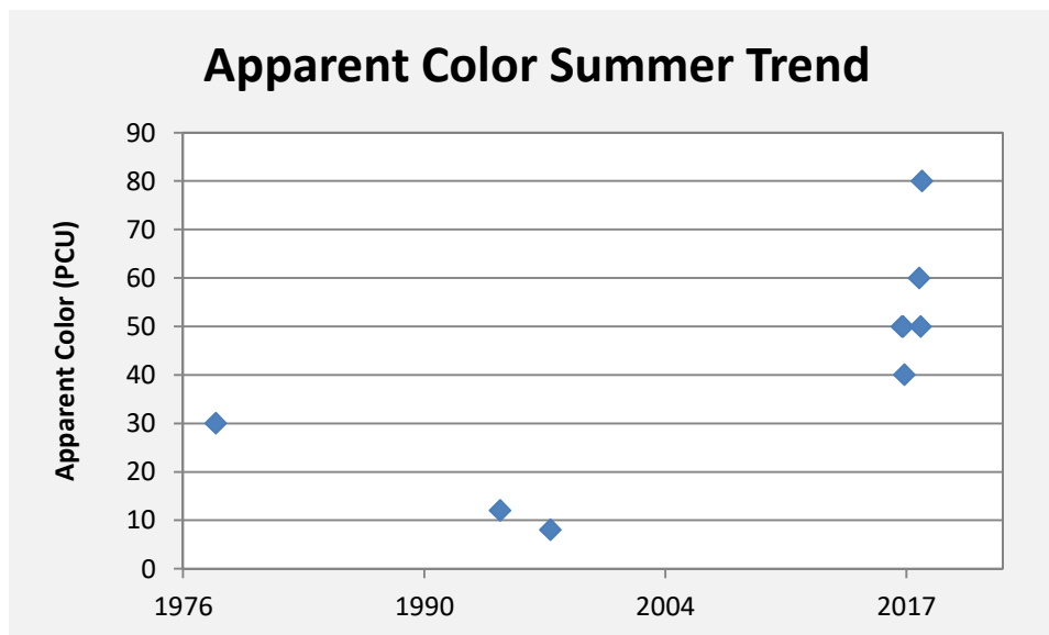
Figure 4.7.3. Historical and recent epilimnion apparent color data for Gregg Lake.
