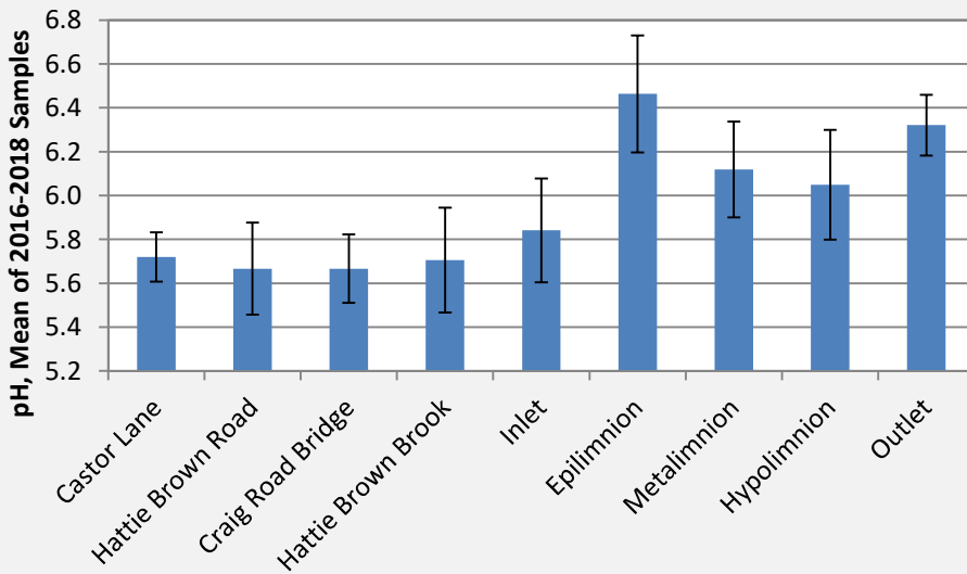
Figure 4.8.3. Mean pH of all samples taken across the full season in 2016–2018. Error bars show the standard deviations for 3-17 samples.
