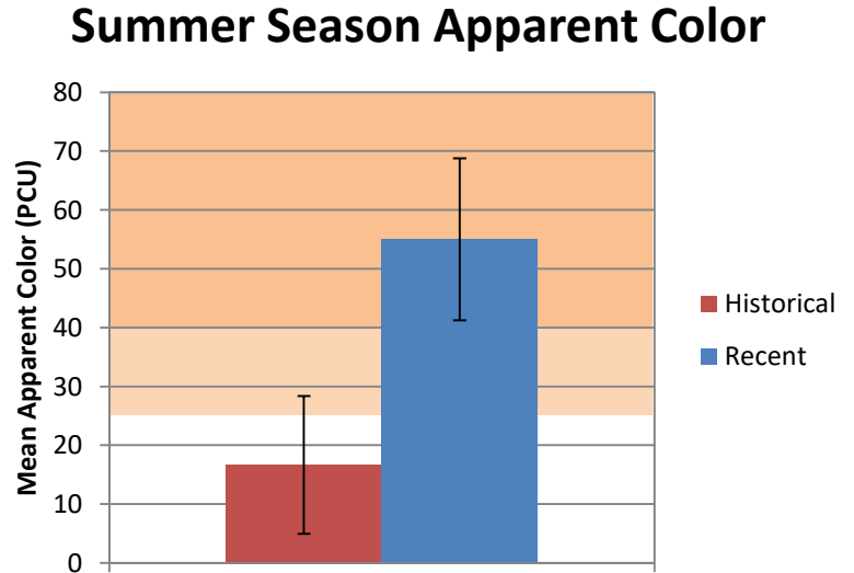
Figure 4.7.2. Mean historical and recent summer apparent color values for the Gregg Lake epilimnion at the Deep Spot. Error bars show standard deviations. Shading shows “Light Tea” and “Tea” color ranges.
