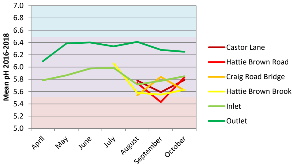
Figure 4.8.2. Mean pH of Inlet, Outlet and Upstream samples collected mid-month in 2016–2018. The satisfactory range is shaded in blue; endangered, in purple; and critical, in red. Data represent single measurements for upstream stations or means of 2-3 samples at the Inlet and Outlet.
